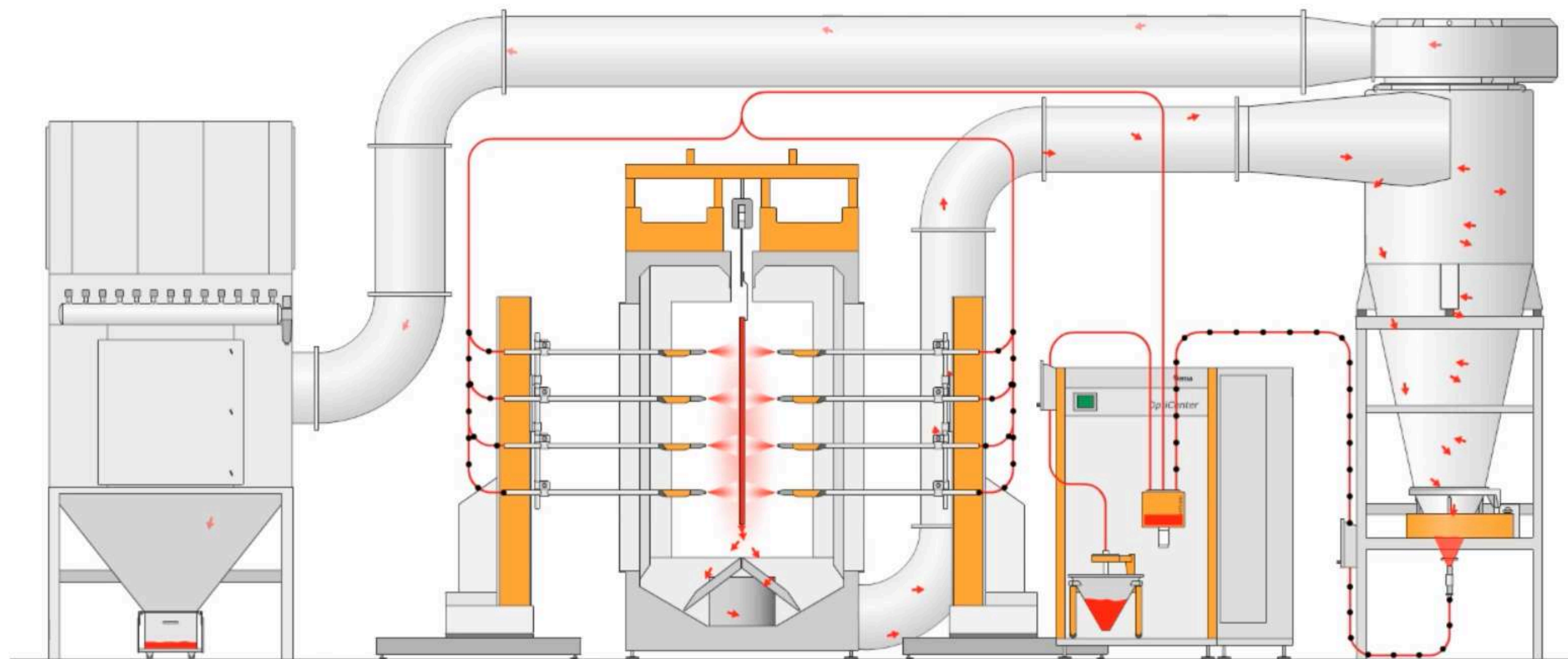
Pollution Free - Powder Coating Circuit
