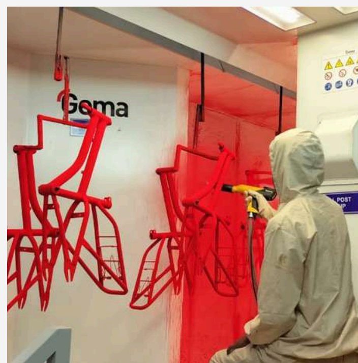
FAST COLOR CHANGE PLASTIC BOOTH
